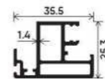
Mosquito Slim Interlock Shutter Section Number : V-2516 Weight (kg/mt) : 0.566
