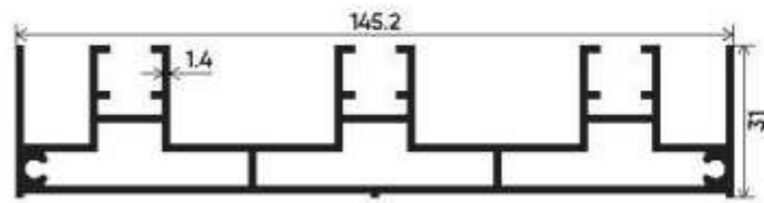
Top & Bottom Track Section Number : V-3505 Weight (kg/mt) : 2.073
