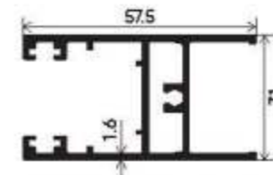
DGU Top Bottom Shutter Section Number : V-3548 Weight (kg/mt) : 0.928
