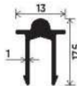
"U" Type Section Number : V-2532 Weight (kg/mt) : 0.166
