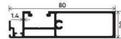
Box Reinforcement Interlock Shutter Section Number : V-2530 Weight (kg/mt) : 0.994
