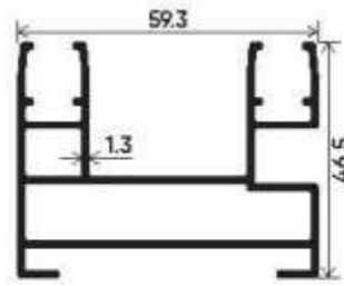
Basic Type Section Number : V-3551 Weight (kg/mt) : 1.048
