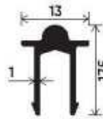
"U" Type Section Number : V-2532 Weight (kg/mt) : 0.166
