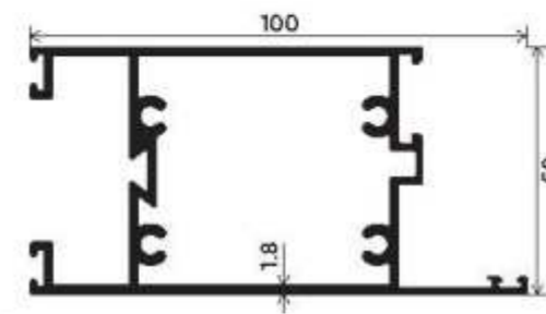
Door Bottom Section Number : V-5005 Weight (kg/mt) : 0.732
