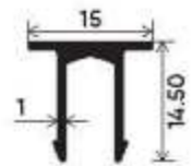
Vertical & Top Track Cover Section Number : V-2533 Weight (kg/mt) : 0.156
