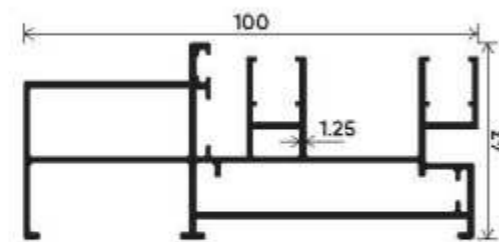
2 in 1 Frame With Grill Section Number : V-2509 Weight (kg/mt) : 1.435
