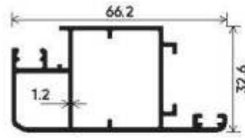
Mesh Shutter Section Number : V-5113 Weight (kg/mt) : 0.779
