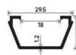
Reducer Clip Laminated Section Number : V-3229 Weight (kg/mt) : 0.195
