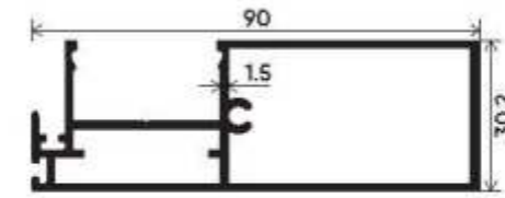
Box Reinforcement Interlock Section Number : V-3227 Weight (kg/mt) : 1.206
