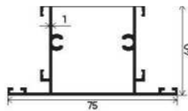
5mm-24mm Glass Shutter Section Number : V-4007/1813 Weight (kg/mt) : 0.947
