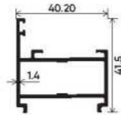
Eco Combination Frame Section Number: V-4032 Weight (kg/mt) : 0.62
