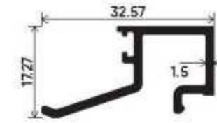
15mm Glass Clip Section Number : V-4036 Weight (kg/mt) : 0.273
