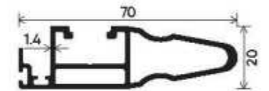
Reinforced Interlock Shutter Section Number : V-2529 Weight (kg/mt) : 0.800
