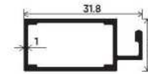
Mosquito Screen Adaptor Section Number : V-3564 Weight (kg/mt) : 0.259
