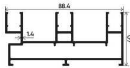
Basic Type Section Number : V-2502 Weight (kg/mt) : 1.417
