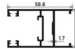
Vertical Shutter Heavy Section Number : V-3514 Weight (kg/mt) : 0.930
