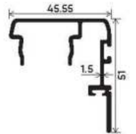
Universal Clip Section Number : V-3771 Weight (kg/mt) : 0.683
