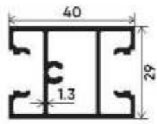
Middle Shutter Section Number : V-2925 Weight (kg/mt) : 0.683
