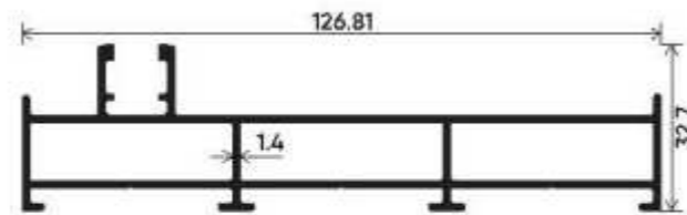
Vertical Track Section Number : V-3105 Weight (kg/m) : 0.941
