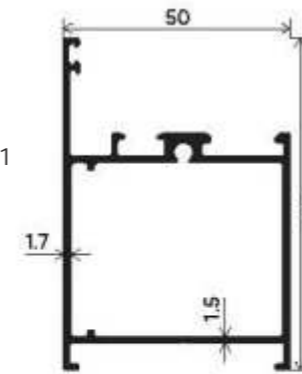
Door Frame Section Number : V-5001 Weight (kg/mt) :1.076
