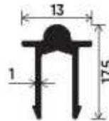
"U" Type Section Number : V-2532 Weight (kg/mt) : 0.166
