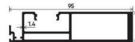
Box Reinforcement SGU Section Number : V-3723 Weight (kg/mt) : 1.317
