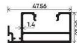
Slim Interlock SGU Section Number : V-3722 Weight (kg/mt) : 0.684
