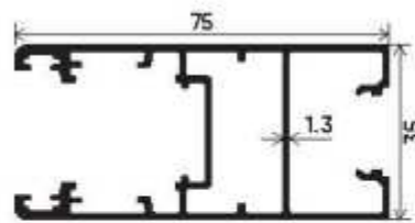
Single Glass Shutter Section Number : V-3561 Weight (kg/mt) : 1.101
