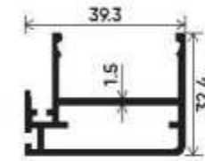
Slim Interlock Shutter 5mm-22mm Glass Shutter Section Number : V-3223 Weight (kg/mt) : 0.596
