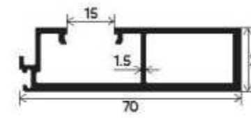
Box Reinforcement Interlock (Laminated Glass) Section Number : V-3542 Weight (kg/mt) : 0.961
