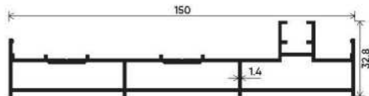
Vertical Track Section Number : V-3503 Weight (kg/mt) : 1.566
