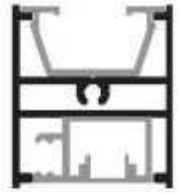
Glass/Mass Middle Section Section Number : V-3521 Weight (kg/mt) : 0.610
