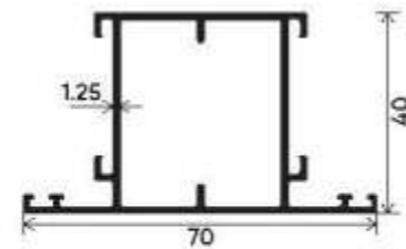
71mm Outside Shutter/Mullion Section Number : V-4004 Weight (kg/mt) : 0.787
