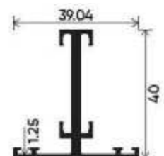
Mullion Section Section Number : V-4022 Weight (kg/mt) : 0.553
