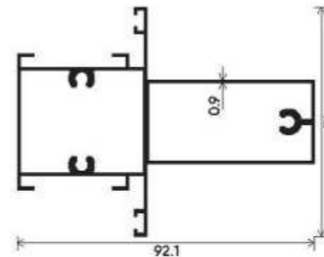
3 In 1 Mullion Section Number :V-4005/1814 Weight (kg/mt) :1.285
