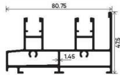
Top & Bottom Track Section Number : V-3103 Weight (kg/m) : 1.640
