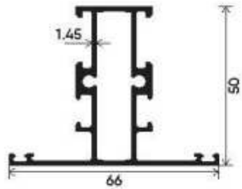
50mm x 65mm Mullion Section Number : V-5103 Weight (kg/mt) :1.089
