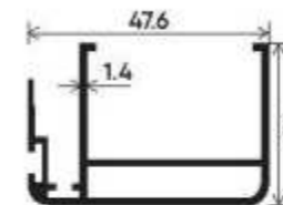
Slim Interlock DGU Section Number : V-3724 Weight (kg/mt) : 0.642
