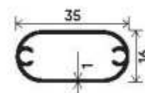
Grill Support Section Number : V-2552 Weight (kg/mt) : 0.276
