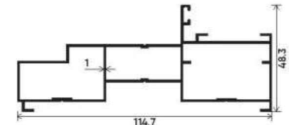
Security Grill & Mosquito Shutter Section Number : V-4002/1810 Weight (kg/mt) :1.338
