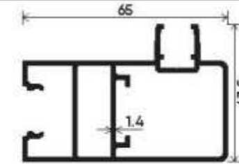
Corner Shutter Section Number : V-3217 Weight (kg/mt) : 1.095
