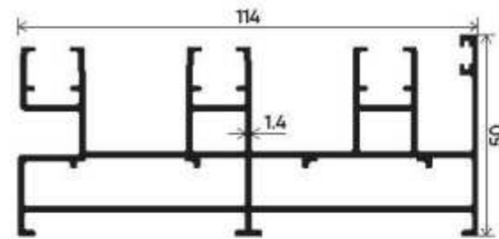
Premium Type Section Number : V-3204 Weight (kg/mt) : 2.099
