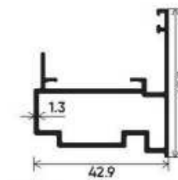
Fly Mullion Section Number : V-4014 Weight (kg/mt) : 0.662
