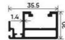
Slim Interlock Shutter Section Number : V-2528 Weight (kg/mt) : 0.495
