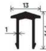
"V" Type Section Number : V-2531 Weight (kg/mt) : 0.156
