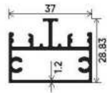
Mosquito Middle Section Section Number : V-292B Weight (kg/mt): 0.592
