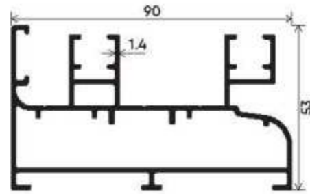
Premium Type Section Number : V-3702 Weight (kg/mt) : 1.640
