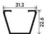
Reducer Clip Section Number : V-3732 Weight (kg/mt) : 0.249
