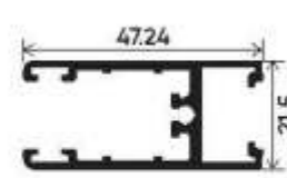
Top & Bottom Shutter Section Number : V-251B Weight (kg/mt) : 0.620
