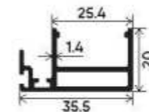
Slim Interlock Shutter 5mm-16mm Glass Shutter Section Number : V-2523 Weight (kg/mt) : 0.468
