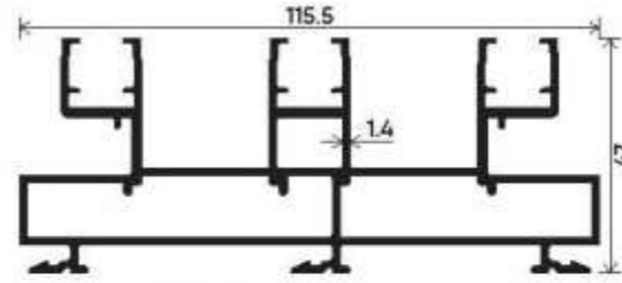
Basic Type Section Number : V-3202 Weight (kg/mt) : 2.206
