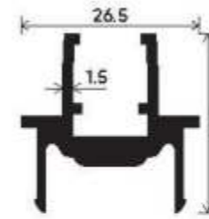
Center Opening Meeting Section Section Number : V-3225 Weight (kg/mt) : 0.464
