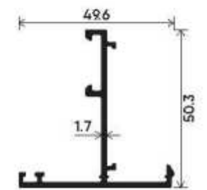
Reverse Adapter Section Number : V-5012 Weight (kg/mt) : 0.497
