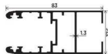
Single Glass Shutter Section Number : V-3711 Weight (kg/mt) : 1.230
