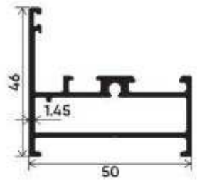
Outer Frame Section Number : V-5101 Weight (kg/mt) : 0.868
