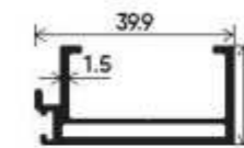
DGU Slim Interlock Section Number : V-3549 Weight (kg/mt) : 0.450
