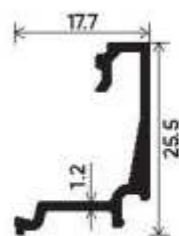
35mm Glass Clip Section Number : V-5015 Weight (kg/mt) : 0.198
