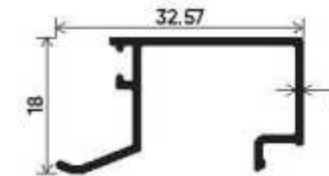
5mm-10mm Glass Clip Section Number: V-4012/1818 Weight (kg/mt) :1.034
