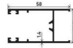
Top & Bottom Shutter Section Number : V-3512 Weight (kg/mt) : 0.683
