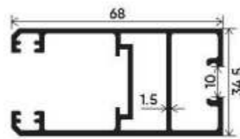
10mm Single Glass Vertical Shutter Section Number : V-3538 Weight (kg/mt) : 1.102
