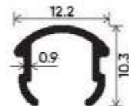
Mosquito Screen Fitting Clip Section Number : V-2524 Weight (kg/12') : 2.900
