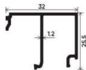
8mm Glass Gap Section Number : V-5009 Weight (kg/mt) : 0.303
