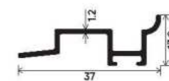
Half Interlock Clip Section Number : V-2520 Weight (kg/mt) : 0.226
