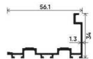
Door Bottom Adapter Section Number : V-5007 Weight (kg/mt) : 0.532
