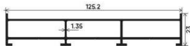
Vertical Track Plain Section Number : V-3107 Weight (kg/m) : 1.300
