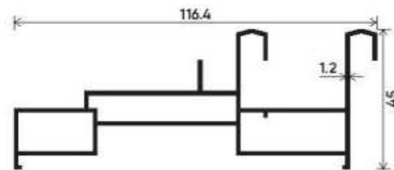
2 Track Grill With Mosquito Section Number : V-2142/1809 Weight (kg/12') : 4.450
