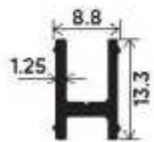
"H" Type Adapter Section Number : V-2534 Weight (kg/mt) : 0.121
