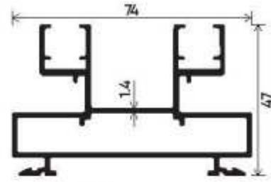
Basic Type Section Number : V-3201 Weight (kg/mt) : 1.444
