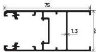
DGU Shutter Section Number : V-3562 Weight (kg/mt) : 1.023
