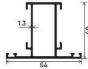
54mm Eco Mullion Section Section Number : V-4003/1770 Weight (kg/mt) : 0.656
