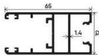
4mm-8mm Glass Shutter Section Number : V-3211 Weight (kg/mt) : 0.950
