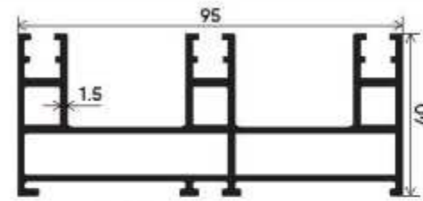
Premium Type Section Number : V-3532 Weight (kg/mt) : 1.870
