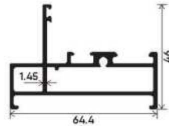
Combination Frame 64mm Section Number : V-5107 Weight (kg/mt) : 0.956
