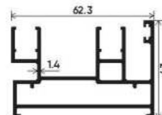
Premium Type Section Number : V-2503 Weight (kg/mt) : 1.168
