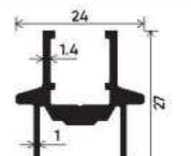
Centre Opening Meeting Section Section Number : V-2525 Weight (kg/mt) : 0.434
