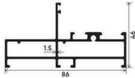
Combination Frame Section Number : V-5104 Weight (kg/mt) :1.654
