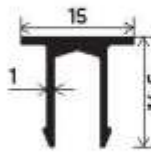
Track Cover Cap Section Number : V-2533 Weight (kg/mt) : 0.140
