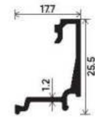
33mm Glass Gap Section Number : V-5015 Weight (kg/mt) : 0.198
