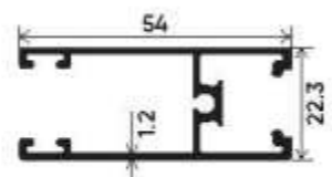
Top Bottom Shutter Section Number : V-2515 Weight (kg/mt) : 0.579
