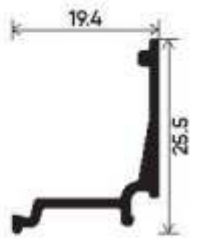
38mm Glass Gap Section Number : V-5013 Weight (kg/mt) : 0.173
