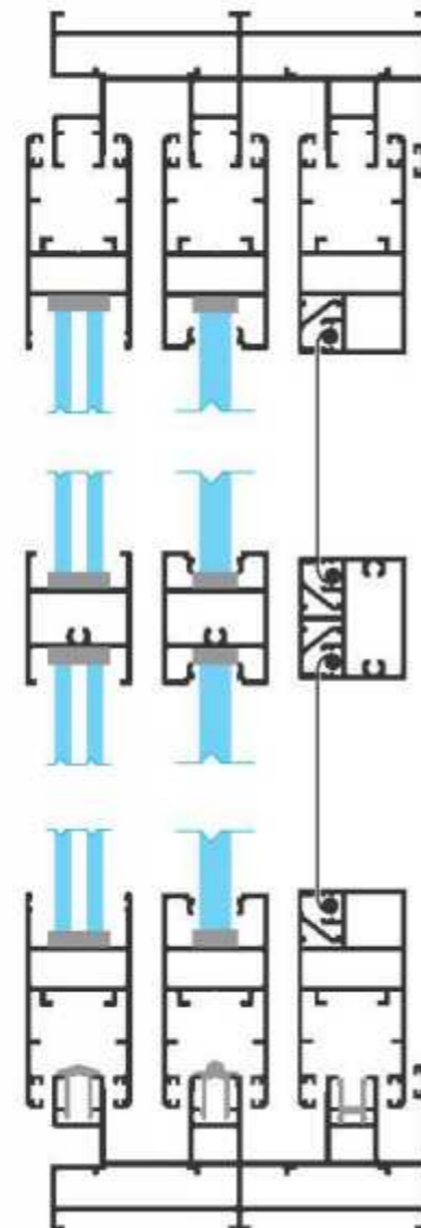
Side View
