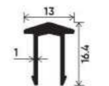
"V" Type Section Number : V-2531 Weight (kg/mt) : 0.156
