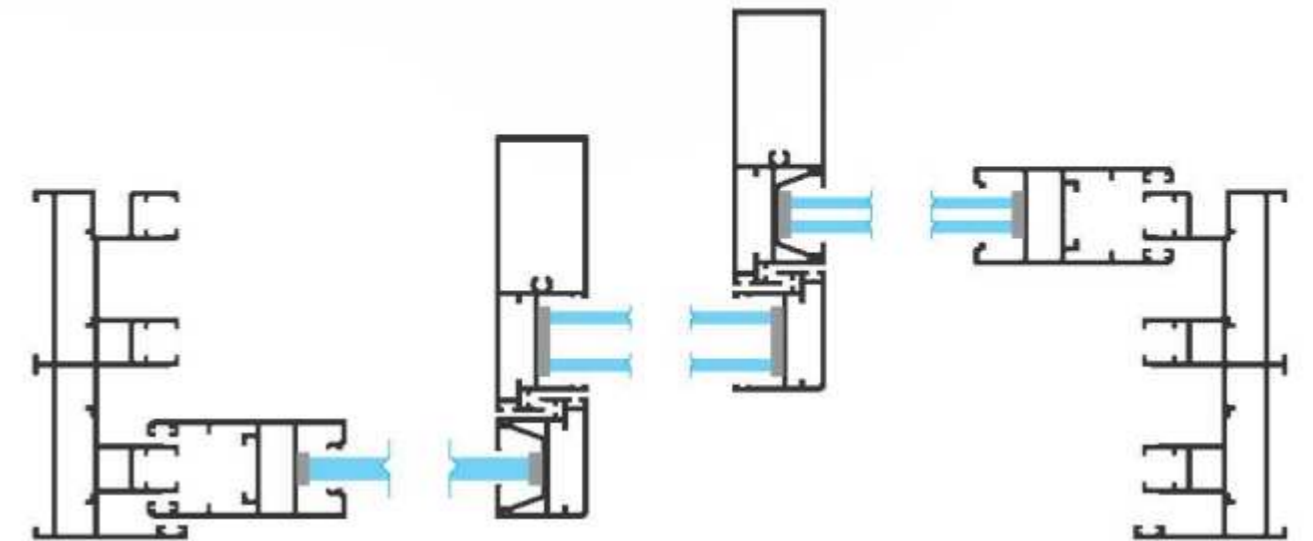
Top View
