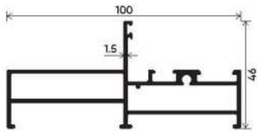
Combination Frame Section Number : V-5105 Weight (kg/mt) :1.336
