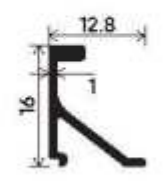
Mosquito Shutter Clip Section Number : V-2514 Weight (kg/mt) : 0.144
