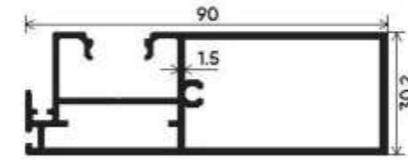
Box Reinforcement Interlock SGU Section Number : V-3228 Weight (kg/mt) : 1.292
