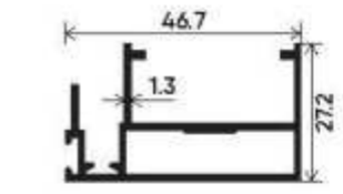
Interlock Section Number : V-3515 Weight (kg/mt) : 0.643
