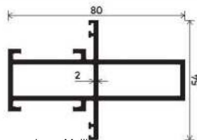
Long Mullion Section Number : V-4034 Weight (kg/mt) :1.455
