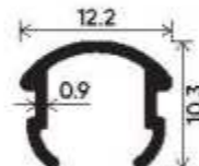
Mosquito Screen Fitting Clip Section Number : V-2524 Weight (kg/mt) : 0.083
