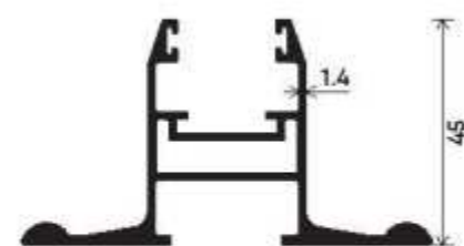
Vertical Shutter DGU Section Number : V-3114 Weight (kg/m) : 1.168
