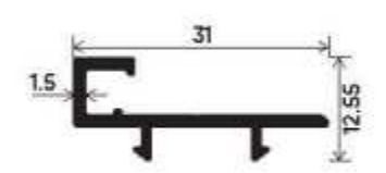
Mosquito Clip Section Number : V-3543 Weight (kg/mt) : 0.20
