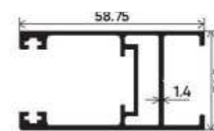
Vertical DGU Shutter Section Number : V-3115 Weight (kg/m) : 0.942
