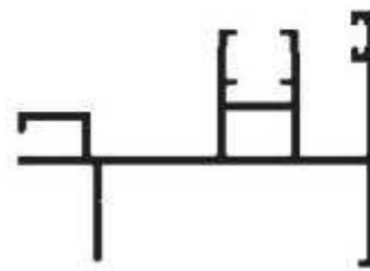
Additional Track Section Number : V-3206 Weight (kg/mt) : 0.689
