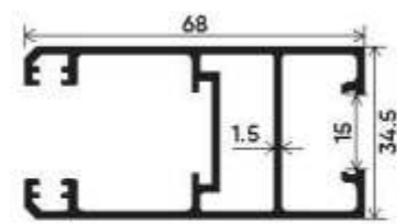
Vertical Shutter (Laminated Glass) Section Number : V-3536 Weight (kg/mt) : 1.066
