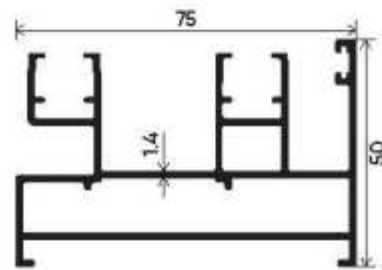
Premium Type Section Number : V-3203 Weight (kg/mt) : 1.409
