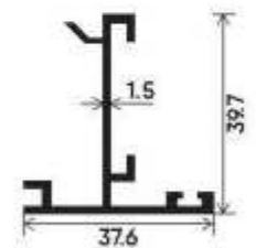
Reverse Adaptor Section Number : V-4015 Weight (kg/mt) : 0.438
