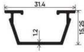
Shutter Glass Reducer Clip Section Number : V-3522 Weight (kg/mt) : 0.211
