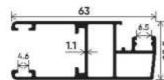
Mosquito screen Shutter Section Number : V-2513 Weight (kg/mt) : 0.793
