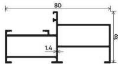
Eco Long Frame Section Number : V-4030 Weight (kg/mt): 0.895
