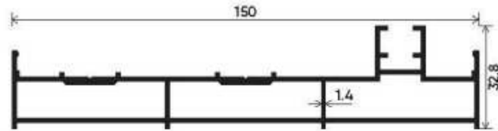
Vertical Track Section Number : V-3503 Weight (kg/mt) : 1.566
