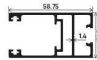
Vertical S. G. Shutter Section Number : V-3111 Weight (kg/m) : 0.942
