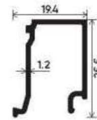
24mm Glass Gap Section Number : V-5008 Weight (kg/mt) : 0.226
