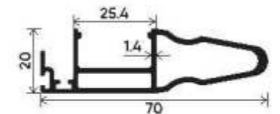
Reinforcement Interlock Shutter 5mm-16mm Glass Shutter Section Number : V-2522 Weight (kg/mt) : 0.803
