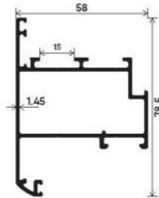
Outside Opening Shutter Section Number: V-5102 Weight (kg/mt) :1.134
