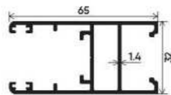
Laminate Shutter Section Number : V-3220 Weight (kg/mt) : 0.910
