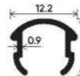
Mosquito Screen Fitting Clip Section Number : V-2524 Weight (kg/mt) : 0.083
