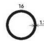
Grill Fitting Tube Cover Section Number : V-1002 Weight (kg/mt) : 0.164
