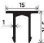
Track Cover Cap Section Number : V-2533 Weight (kg/mt) : 0.140
