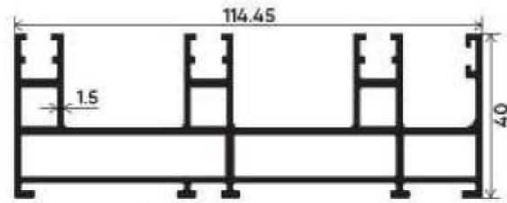
Premium Type Section Number : V-3531 Weight (kg/mt) : 2.150
