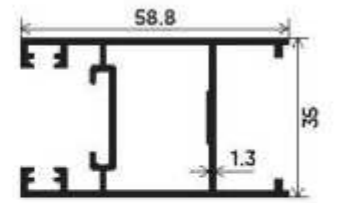
Vertical Shutter Premium Section Number : V-3530 Weight (kg/mt) : 0.891
