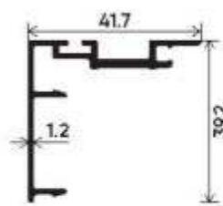
Universal Clip Section Number : V-3571 Weight (kg/mt) : 0.409
