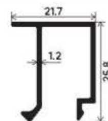
19mm Glass Gap Section Number : V-5011 Weight (kg/mt) : 0.241
