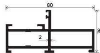
Eco Long Frame Section Number : V-4033 Weight (kg/mt) :1.414
