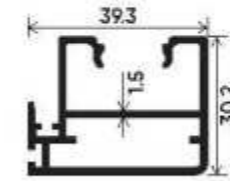
Slim Interlock Shutter SGU Section Number : V-3224 Weight (kg/mt) : 0.692
