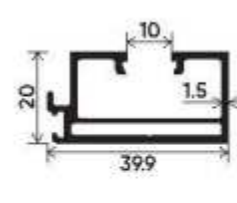
10mm Single Glass Slim Interlock Section Number : V-3544 Weight (kg/mt) : 0.544
