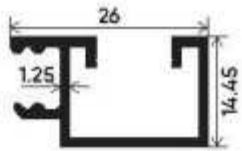
Mosquito Screen Adaptor Section Number : V-3524 Weight (kg/mt) : 0.242
