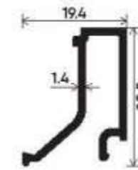
30mm Glass Gap Section Number : V-5014 Weight (kg/mt) : 0.247
