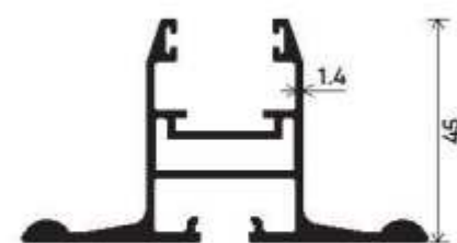
Vertical Shutter SGU Section Number : V-3113 Weight (kg/m) : 1.100
