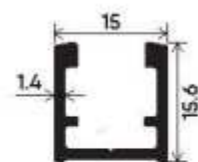
Locking Adapter Section Number : V-3106 Weight (kg/m) : 0.199
