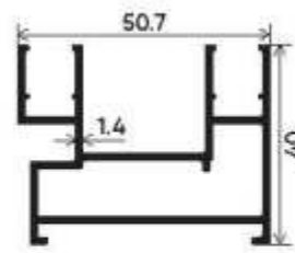
Basic Type Section Number : V-2501 Weight (kg/mt) : 0.883
