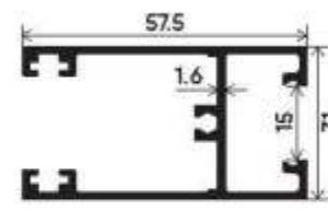
Top Bottom Shutter (Laminated Glass) Section Number : V-3537 Weight (kg/mt) : 0.869
