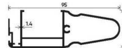
Box Reinforcement DGU Section Number : V-3725 Weight (kg/mt) : 1.085
