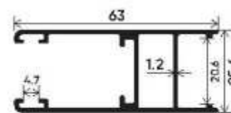
5mm-16mm Glass Shutter Section Number : V-2512 Weight (kg/mt) : 0.725
