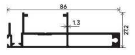
40mm Reinforcement Interlock Shutter Section Number : V-3517 Weight (kg/mt) : 0.977
