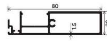
Box Reinforcement Interlock Section Number : V-2527 Weight (kg/mt) : 0.929
