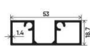
Premium Bottom Guide Section Number : V-5205 Weight (kg/mt) : 0.660
