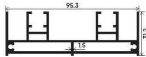
Top & Bottom Track Section Number : V-3502 Weight (kg/mt) : 1.544
