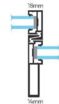
Section Detail
