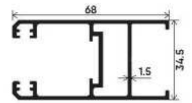
DGU Vertical Shutter Section Number : V-3547 Weight (kg/mt) : 1.000
