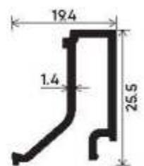
30mm Glass Clip Section Number : V-5014 Weight (kg/mt) : 0.247
