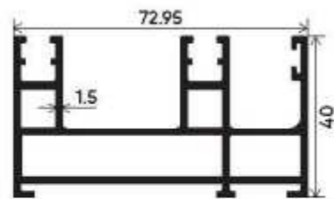
Premium Type Section Number : V-3533 Weight (kg/mt) : 1.478
