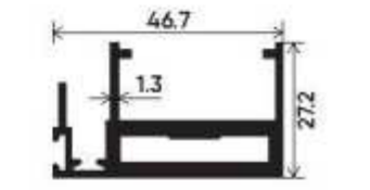
Interlock Heavy Section Number : V-3526 Weight (kg/mt) : 0.989
