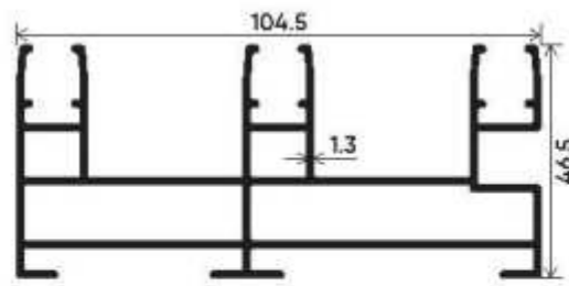
Basic Type Section Number : V-3555 Weight (kg/mt) : 1.722
