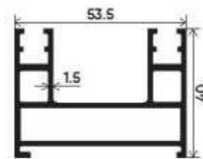
Basic Type Section Number : V-3534 Weight (kg/mt) : 1.110
