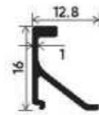
Mosquito Shutter Clip Section Number : V-2514 Weight (kg/mt) : 0.144
