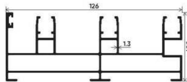
Premium Type Section Number : V-3556 Weight (kg/mt) : 1.950
