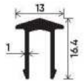
"V" Type Section Number : V-2531 Weight (kg/mt) : 0.156
