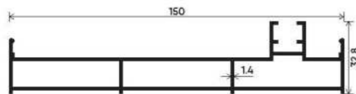
Plain Vertical Track Section Number : V-3510 Weight (kg/mt) : 1.566
