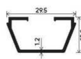
Reducer Clip SGU Section Number : V-3226-1 Weight (kg/mt) : 0.225
