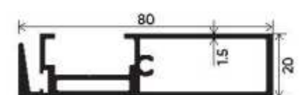
Box Reinforcement Interlock DGU Section Number : V-3118 Weight (kg/m) : 1.202
