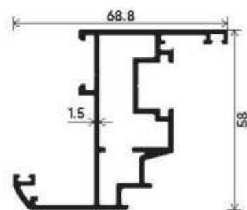
Tilt & Turn Section Number : V-5111 Weight (kg/mt) :1.133
