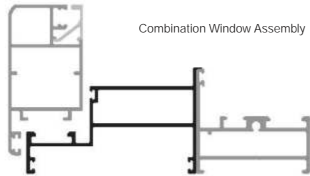
Combination Frame Section Number : V-5112 Weight (kg/mt) : 0.859
