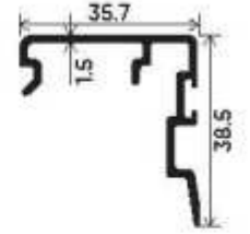
Universal Clip Section Number : V-3221 Weight (kg/mt) : 0.561
