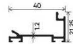
Shutter Bottom Clip Section Number : V-4016 Weight (kg/mt) : 0.308
