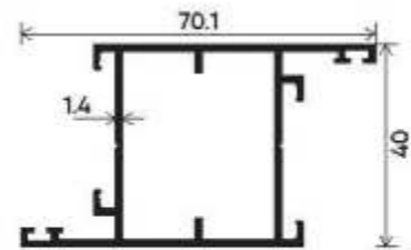
Inside Opening Shutter Section Number : V-4031 Weight (kg/mt) :1.346
