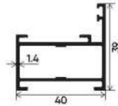
Eco Cutter Frame Section Number : V-4001/1816 Weight (kg/mt) : 0.410
