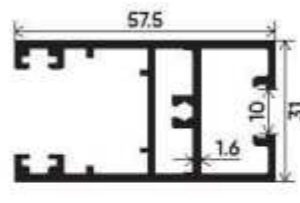
10mm Single Glass Top Bottom Shutter Section Number : V-3539 Weight (kg/mt) : 1.033
