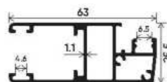
Mosquito Shutter with Scru Pocket Section Number : V-2517 Weight (kg/mt) : 0.900
