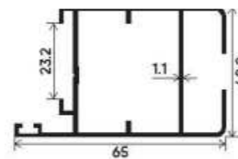
Mosquito screen Shutter Section Number : V-4008/1811 Weight (kg/mt) : 0.929
