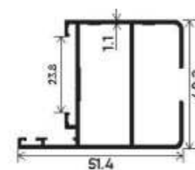
Single Glass Middle Section Number : V-4009/1815 Weight (kg/mt) : 0.742
