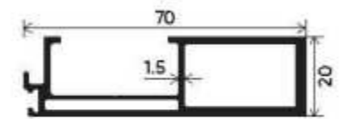
DGU Box Reinforcement Interlock Section Number : V-3550 Weight (kg/mt) : 0.884
