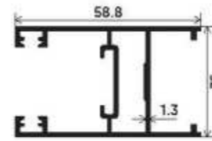
Vertical Shutter Section Number : V-3511 Weight (kg/mt) : 0.891
