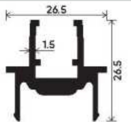
Center Opening Meeting Section Section Number : V-3225 Weight (kg/mt) : 0.464
