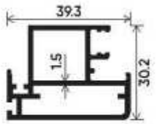
Mosquito Slim Interlock Shutter Section Number : V-3216 Weight (kg/mt) : 0.727
