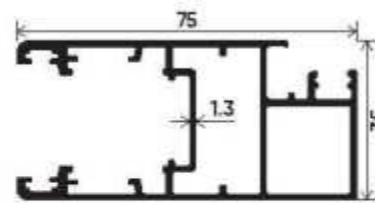
Mosquito Shutter Section Number : V-3563 Weight (kg/mt) : 1.123
