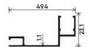
Mosquito Shutter Track Bracket Section Number : V-2510 Weight (kg/mt) : 0.345
