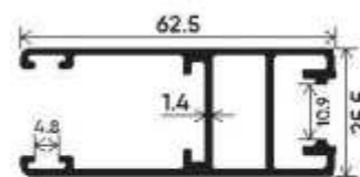
4mm-8mm Single Glass Shutter Section Number : V-2511 Weight (kg/mt) : 0.835
