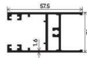
DGU Top Bottom Shutter Section Number : V-3548 Weight (kg/mt) : 0.928
