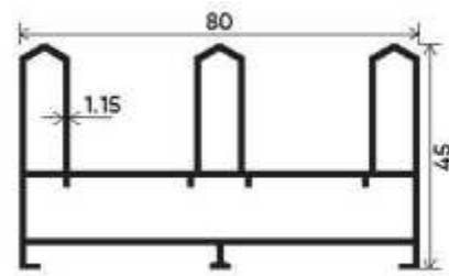
Regular Type Section Number : V-2717 Weight (kg/12') : 4.280
