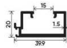
Slim Interlock Shutter (Laminated Glass) Section Number : V-3541 Weight (kg/mt) : 0.525
