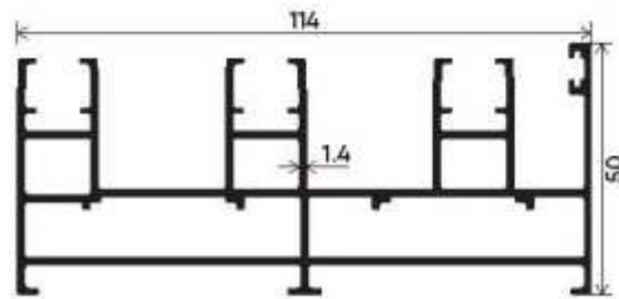
Premium Type Plain Section Number : V-3207 Weight (kg/mt) : 2.100
