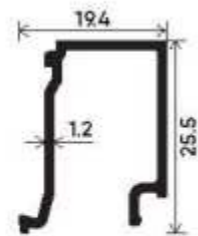
18mm-24mm Glass Clip Section Number : V-5008 Weight (kg/mt) : 0.226
