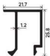
10mm-16mm Glass Clip Section Number : V-5011 Weight (kg/mt) : 0.241
