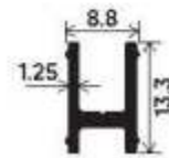
"H" Type Adapter Section Number : V-2534 Weight (kg/mt) : 0.121
