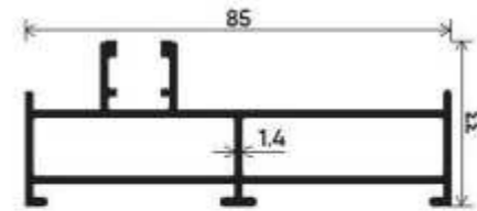
Vertical Track Section Number : V-3102 Weight (kg/m) : 1.04
