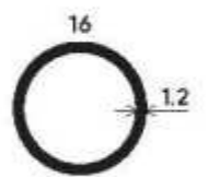
Grill Fitting Tube Cover Section Number : V-1002 Weight (kg/mt) : 0.164
