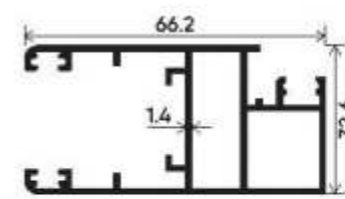
Mosquito Screen Shutter Section Number : V-3213 Weight (kg/mt) : 0.894
