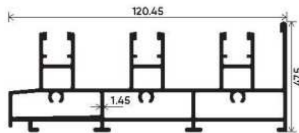
Top & Bottom Track Section Number : V-3104 Weight (kg/m) : 2.281
