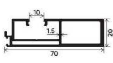
10mm Single Glass Box Reinforcement Interlock Section Number : V-3545 Weight (kg/mt) : 0.988
