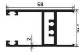
Top & Bottom Shutter Heavy Section Number : V-3529 Weight (kg/mt) : 1.000
