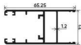
5mm-24mm Glass Shutter Section Number : V-3212 Weight (kg/mt) : 0.947
