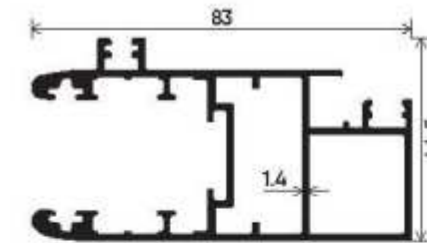
Mosquito Shutter Section Number : V-3713 Weight (kg/mt) : 1.240
