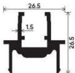
Center Opening Meeting Section Section Number : V-3225 Weight (kg/mt) : 0.464
