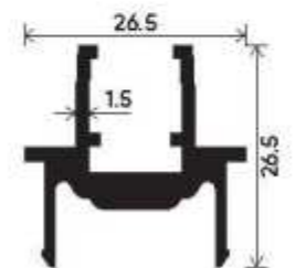
Center Opening Meeting Section Section Number : V-3731 Weight (kg/mt) : 0.469
