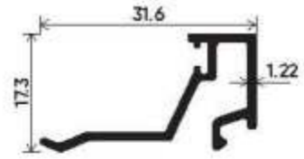
18mm-24mm Glass Clip Section Number : V-4013 Weight (kg/mt) : 0.561
