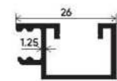
Mosquito Screen Adaptor Section Number : V-3524 Weight (kg/mt) : 0.242
