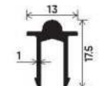
"U" Type Section Number : V-2532 Weight (kg/mt) : 0.166
